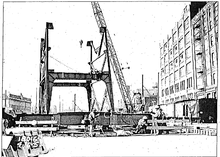
Construction of Alaskan Way Viaduct at Pike November 15, 1949 Item 43037 Seattle Municipal Archives
