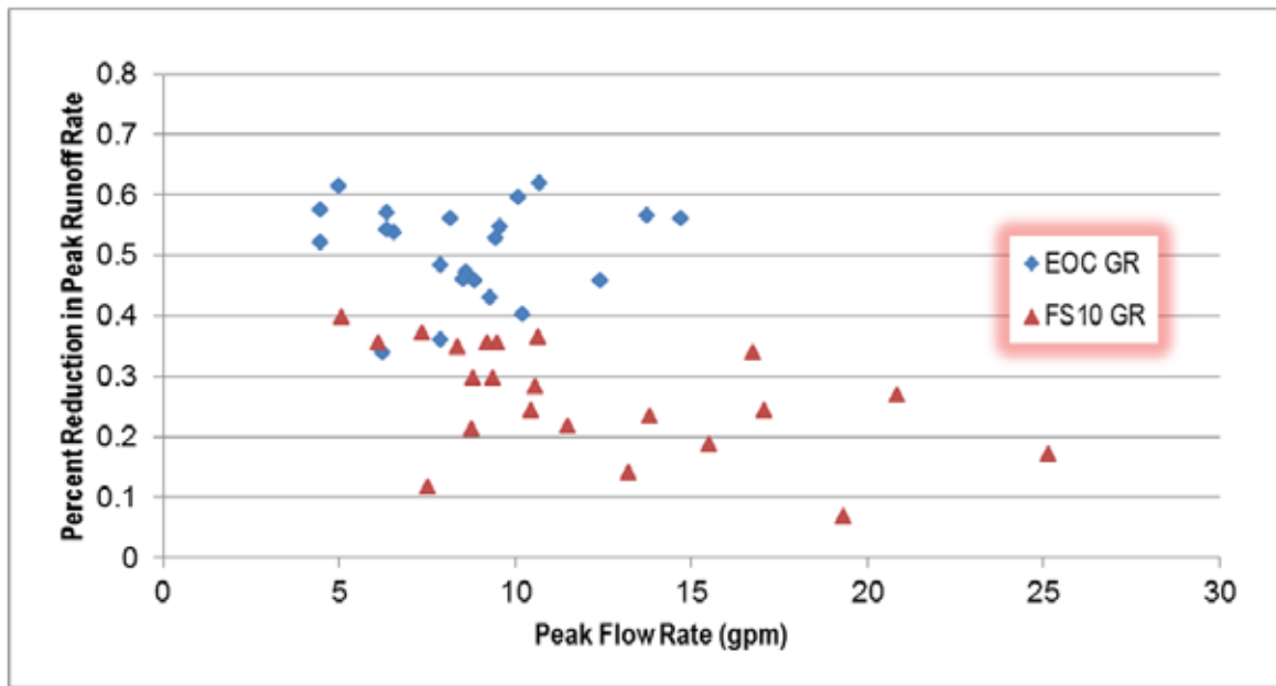
Figure 5-1 Percent Peak Run-off Reduction for Selected Events
