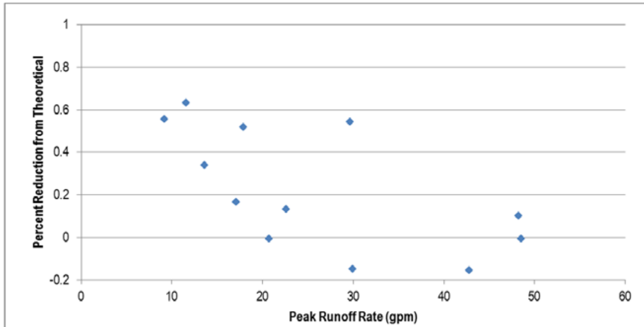
Figure 5-3 Percent Peak Runoff Reduction for Selected Zoomazium Events
