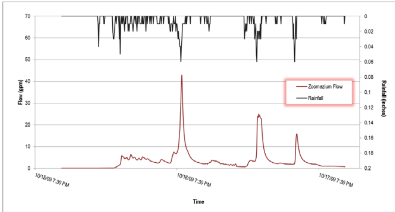
Figure 5-5 Zoomazium Rainfall-Runoff Response in Successive Events
