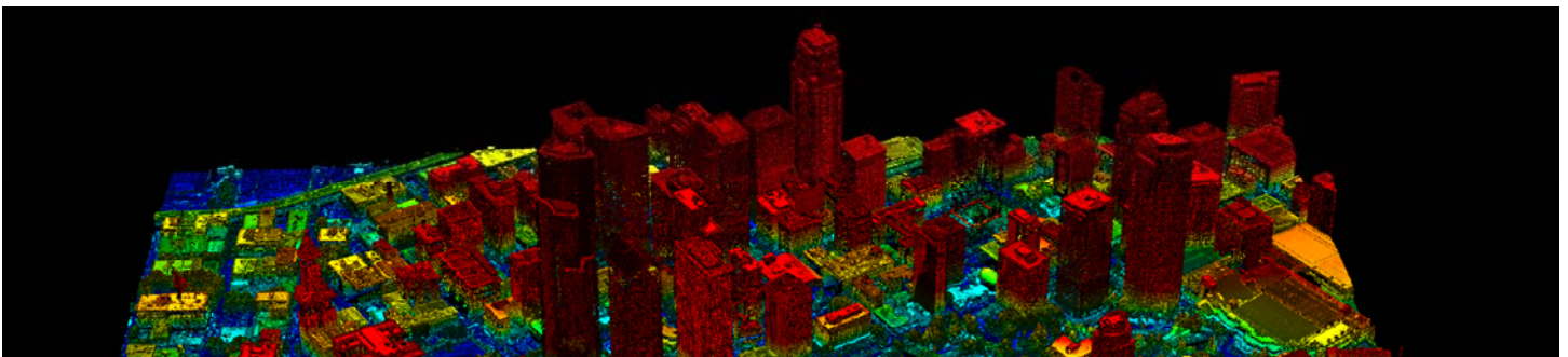
Figure 25. 2016 LiDAR for Seattle. The acquisition of such data in the future will be crucial for tracking tree canopy change over time.
